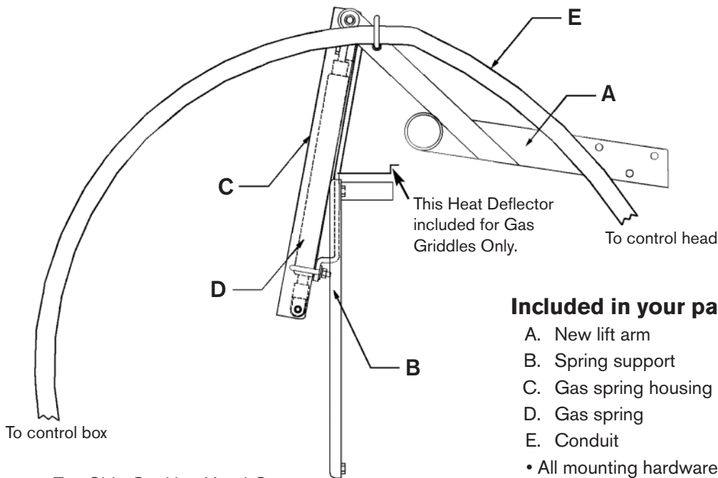
Top-Side Cooking Head Cover
